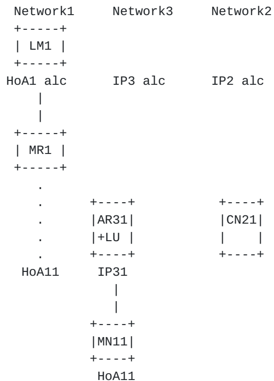
Figure 2. Functional decomposition of PMIPv6
