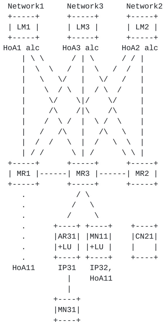
Figure 9. DMM with Control and Data Plane Separation
