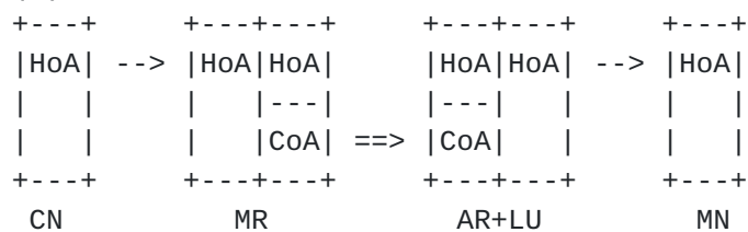
Figure 3. Network layer in the protocol stack of packets sent from the CN and tunneled (a) to the MN+LU in MIPv6; and (b) to the AR+LU in PMIPv6 showing the destination IP address as the packet traverses from the CN to the MN.
