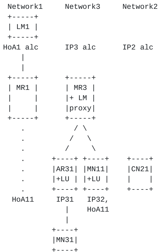
Figure 4. Functional decomposition of Hierarchical Mobile IPv6
