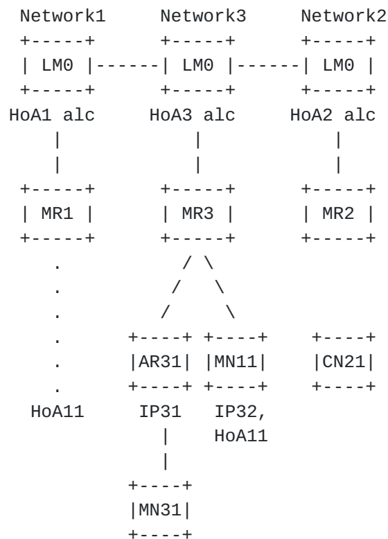
Figure 6. Functional decomposition of Migrating Home Agents
