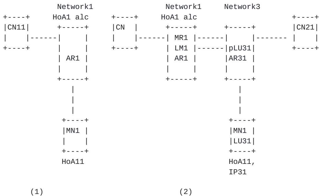
Figure 7. Client-based DMM architecture for a flat network.
