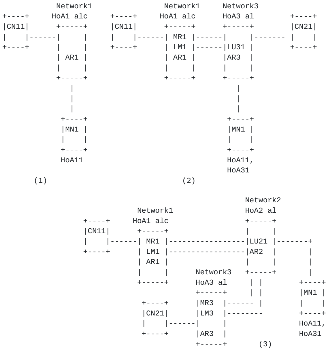
Figure 6. Network-based DMM architecture for a flat network.
