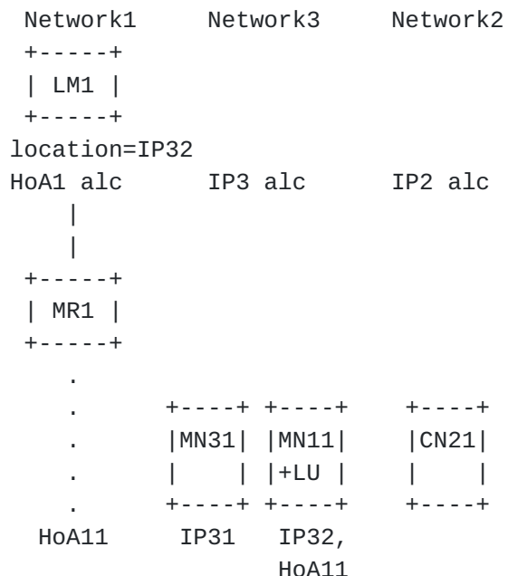
Figure 1. Functional decomposition of Mobile IPv6.
