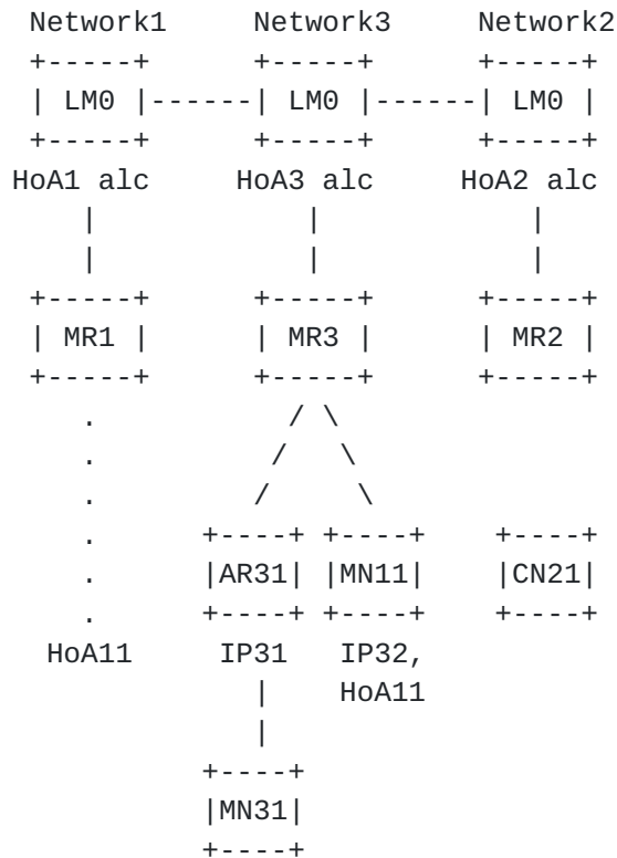
Figure 5. Functional representation of Migrating Home Agents.
