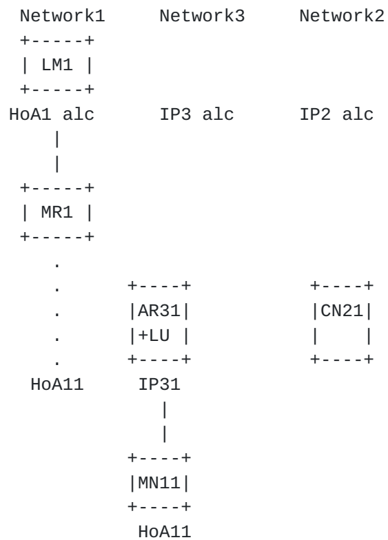
Figure 3. Functional representation of PMIPv6.
