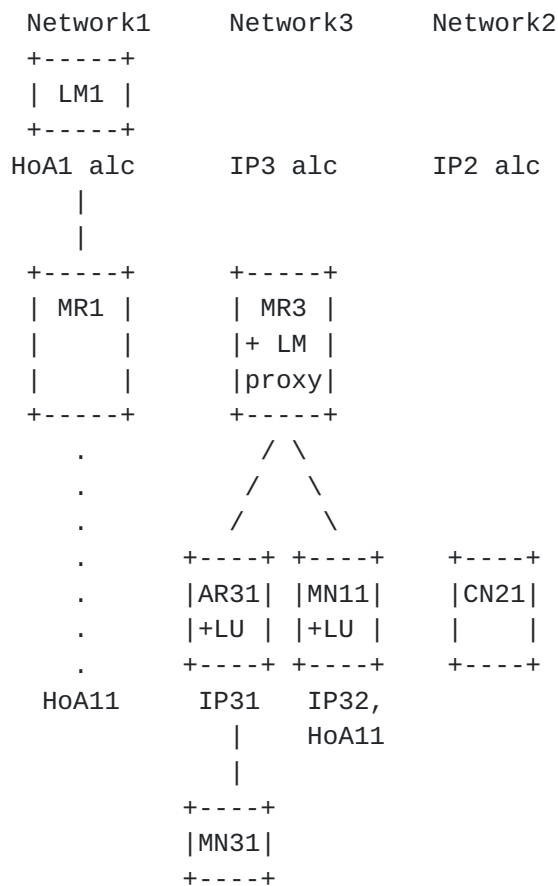
Figure 4. Functional representation of Hierarchical Mobile IPv6.
