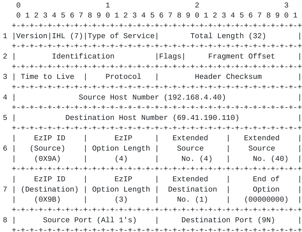
Figure 33 TCP/EzIP Header: From T4z to SPR4
