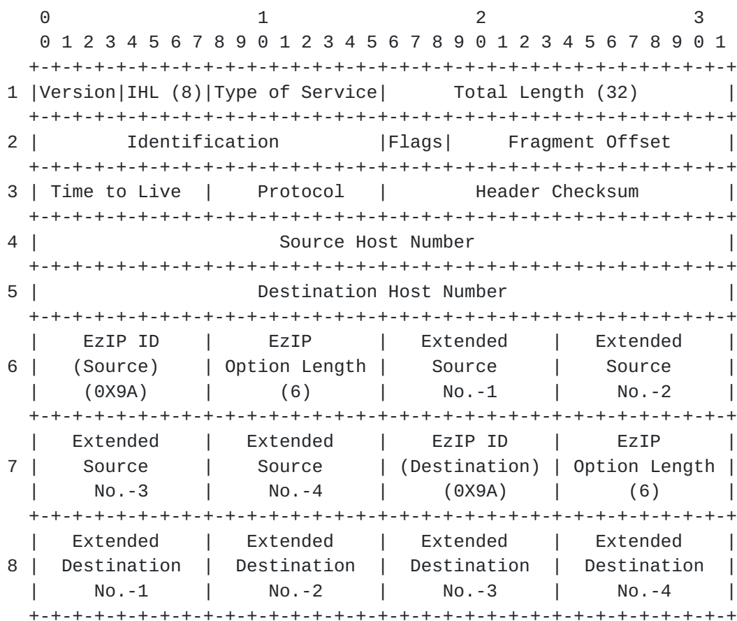
Figure 14 Full EzIP Header (Four octet)
