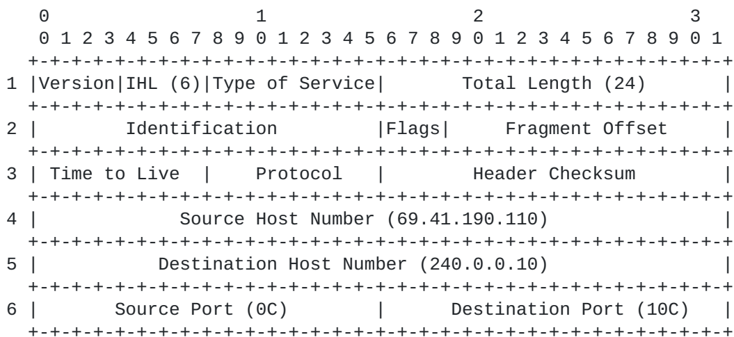
Figure 8 TCP/IP Header: From SPR4 to T4a
