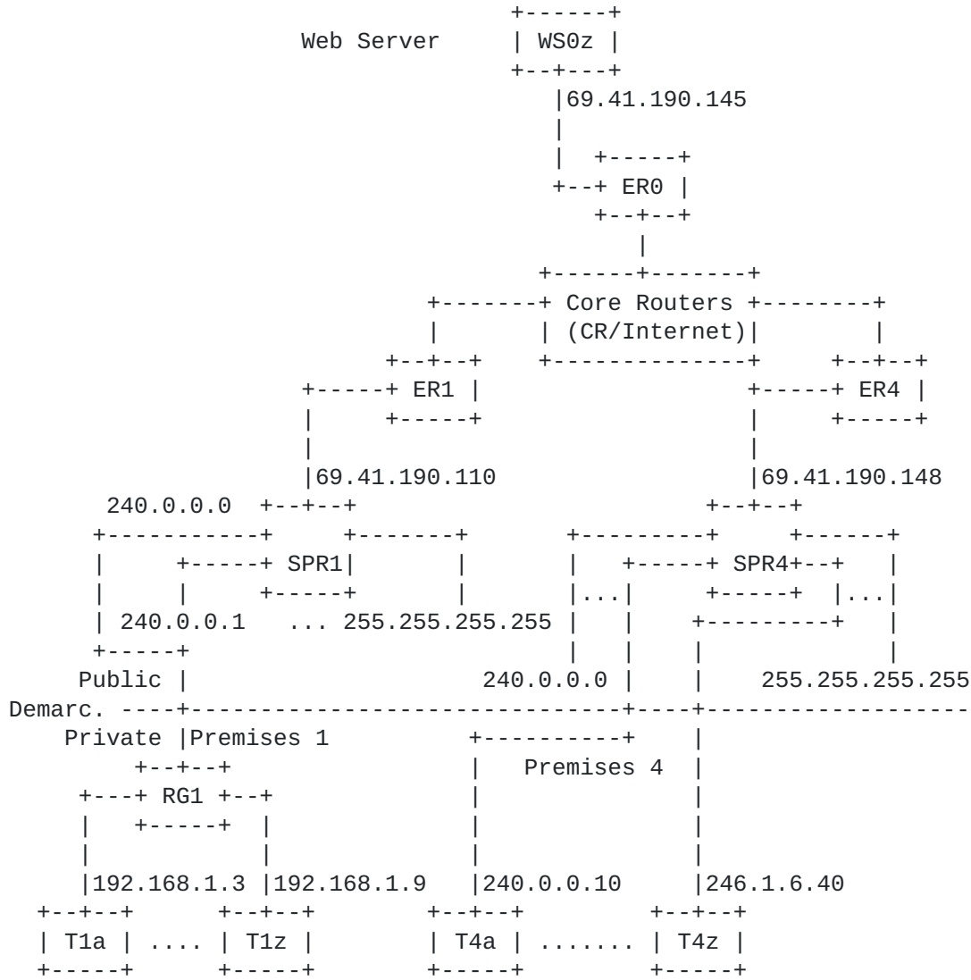
Figure 1 EzIP System Architecture
