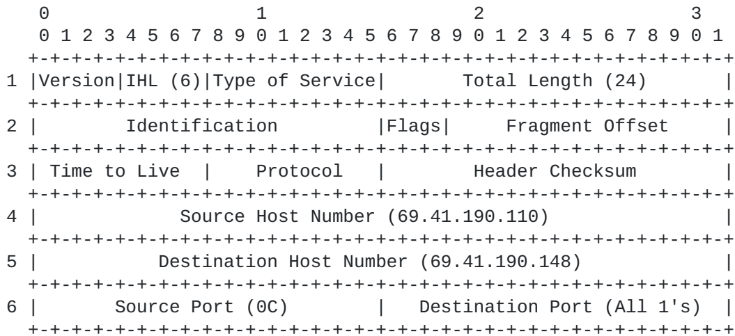
Figure 7 TCP/IP Header: From SPR1 to SPR4
