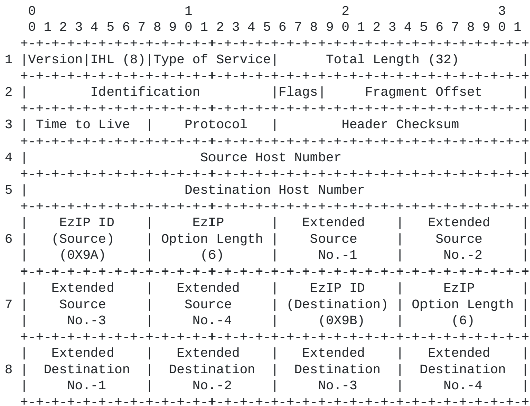
Figure 4 Full EzIP Header
