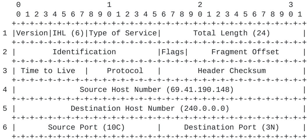
Figure 11 TCP/IP Header: From SPR1 to RG1
