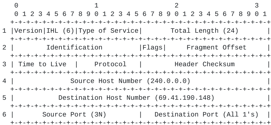
Figure 6 TCP/IP Header: From RG1 to SPR1
