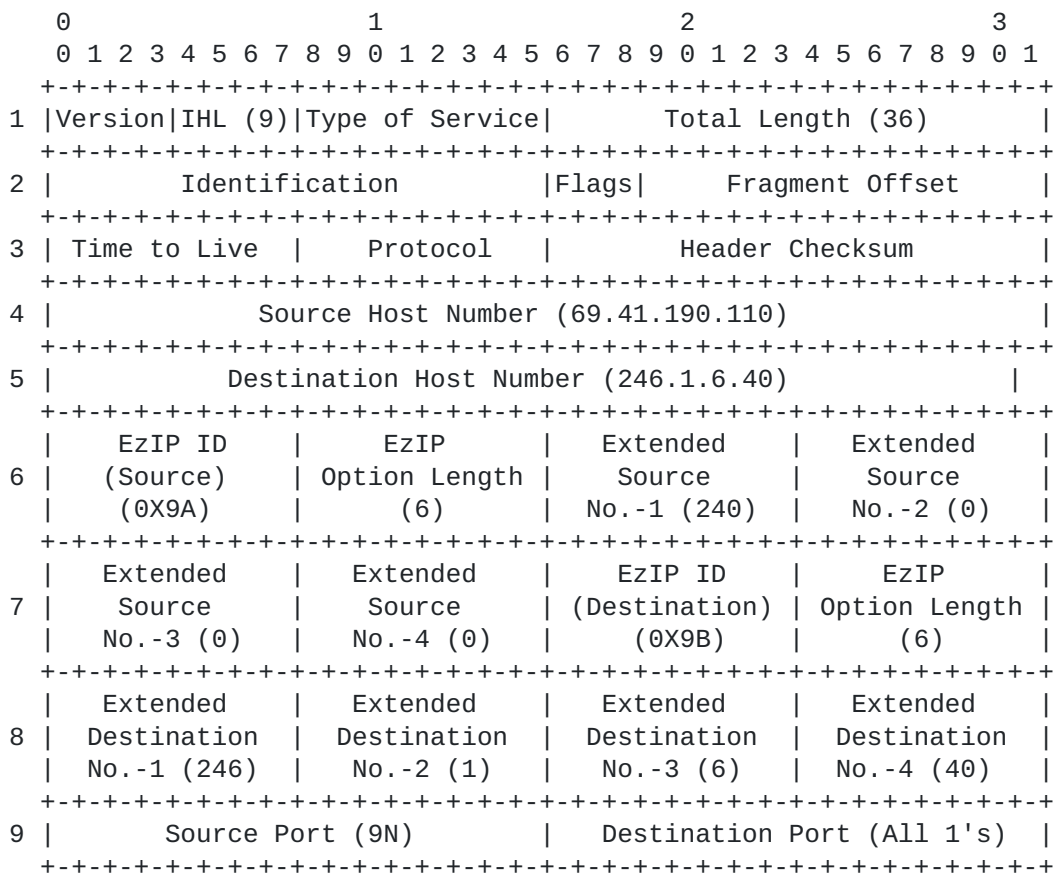
Figure 17 TCP/EzIP Header: From SPR4 to T4z
