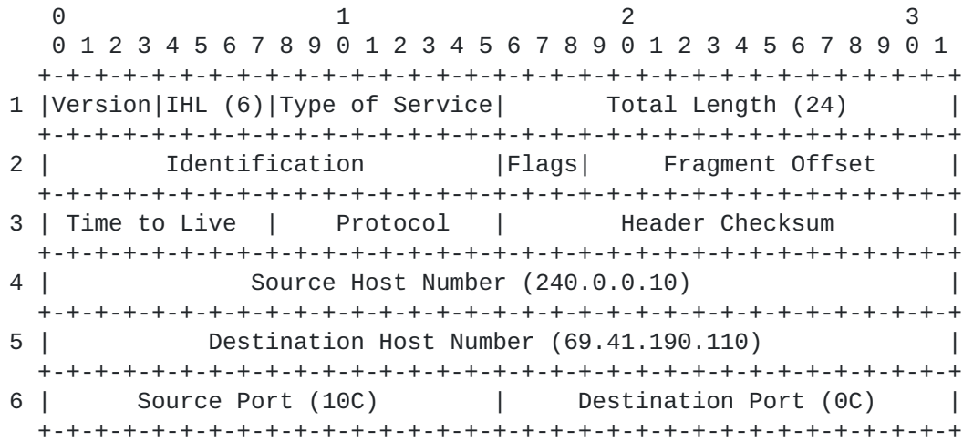
Figure 9 TCP/IP Header: From T4a to SPR4
