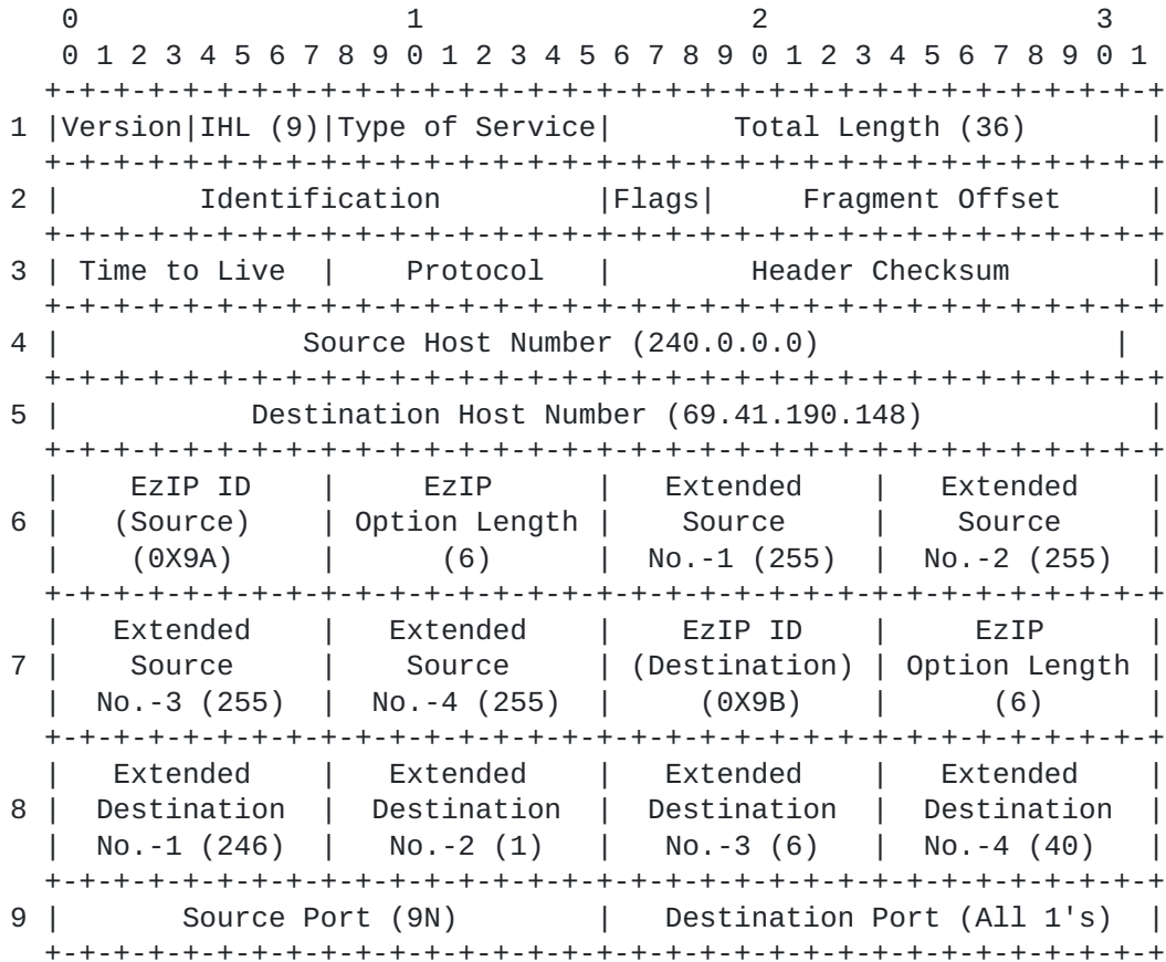
Figure 15 TCP/EzIP Header: From RG1 to SPR1
