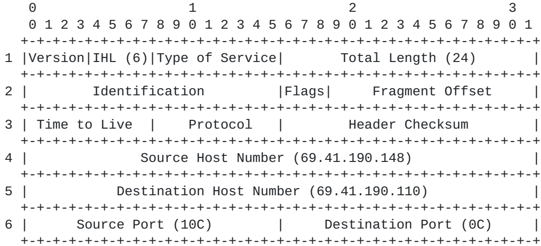
Figure 10 TCP/IP Header: From SPR4 to SPR1
