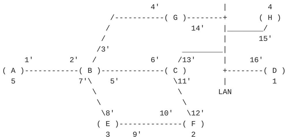
Figure 1: Example BIER-TE Topology with BP to BFR on LAN
