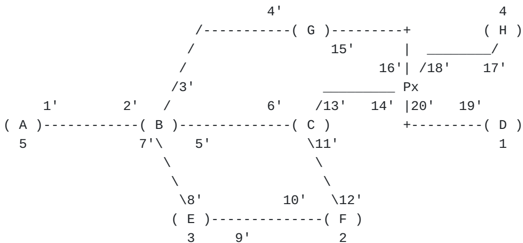
Figure 10: Example BIER-TE Topology with BPs for LAN
