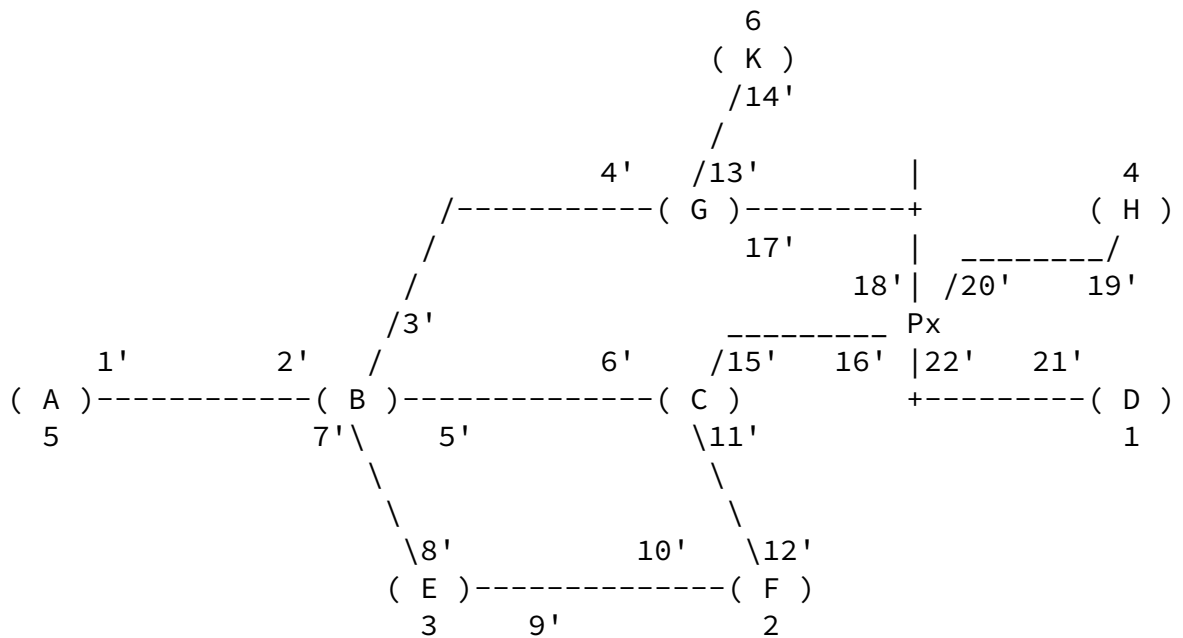
Figure 10: Example BIER-TE Topology with BPs for LAN
