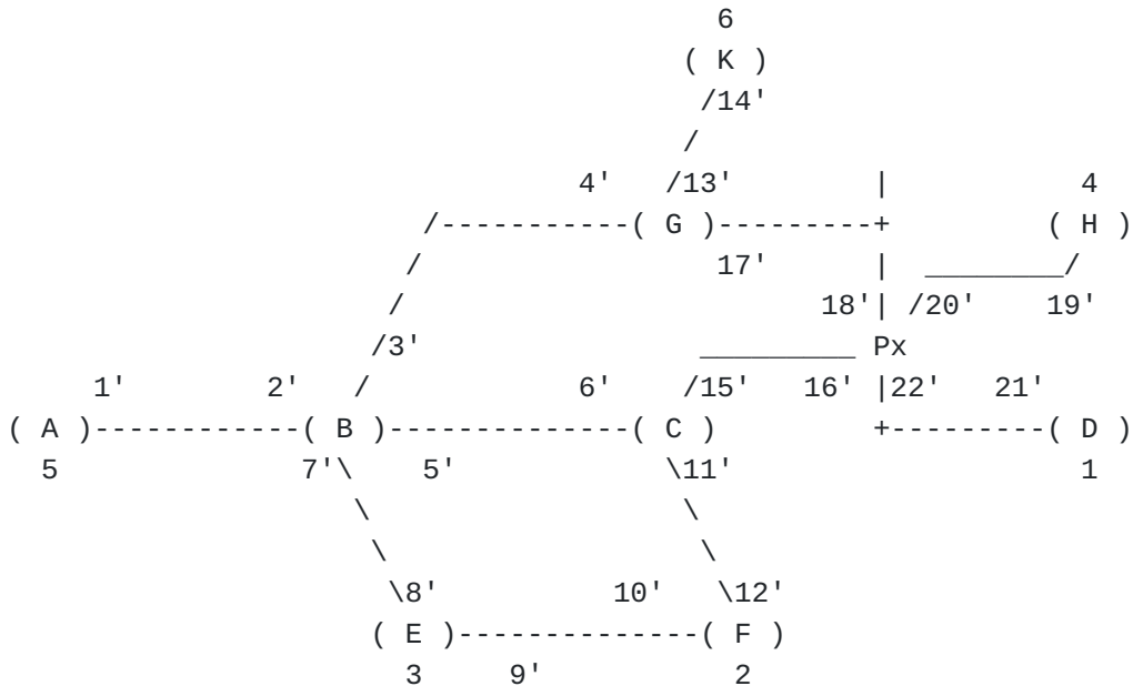
Figure 10: Example BIER-TE Topology with BPs for LAN
