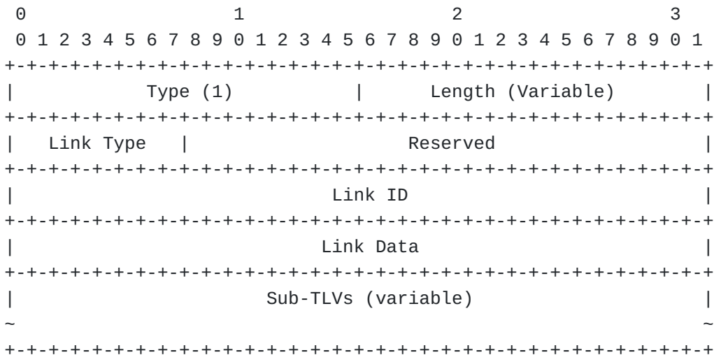
Figure 1: OSPFv2 Extended Link TLV
