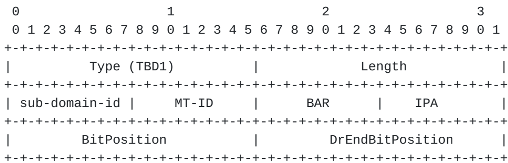
Figure 1: BIER-TE Sub-TLV in Router-Link TLV
