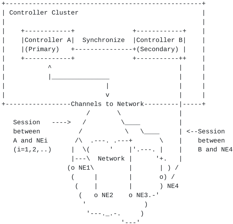
Figure 1: Controller Cluster of 2 Controllers
