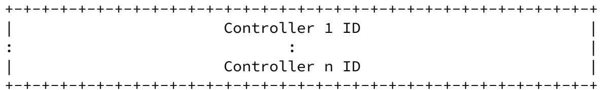
Figure 2: OSPF Controllers TLV
