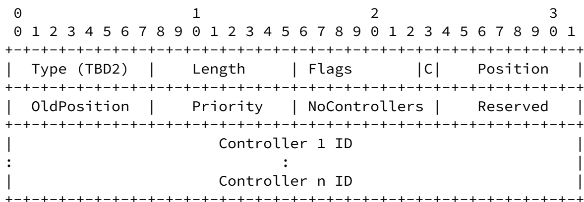
Figure 3: IS-IS Controllers TLV
