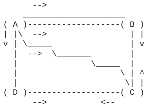
Figure 2: BGP-SPF Domain with parallel links
