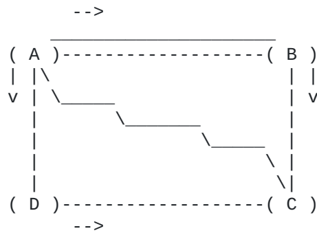
Figure 4: A Reduced Link State Flooding Flow
