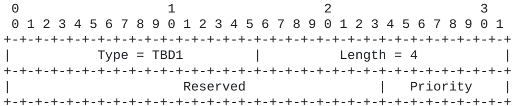
Figure 5: Leader Priority TLV
