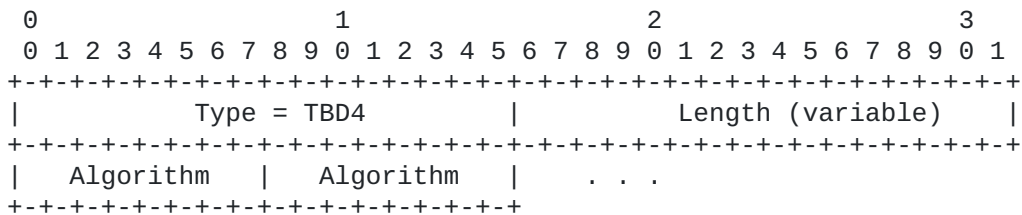
Figure 8: Algorithms Support TLV
