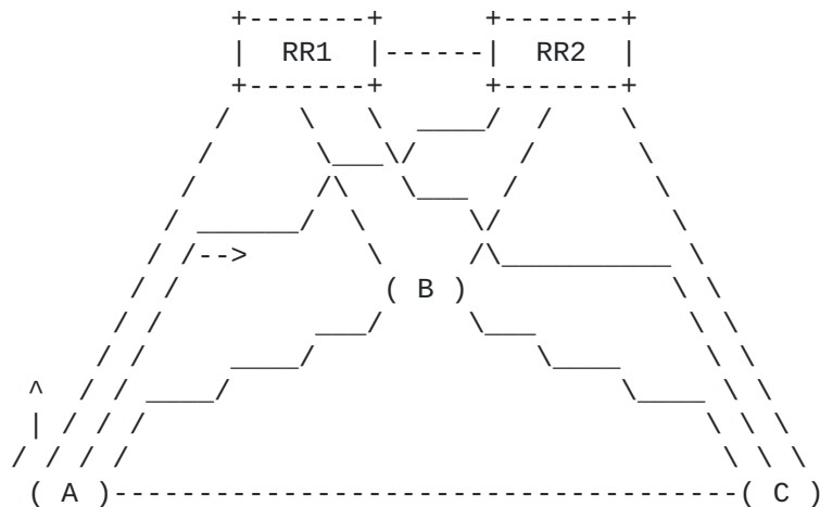
Figure 1: BGP-SPF Domain with two RRs
