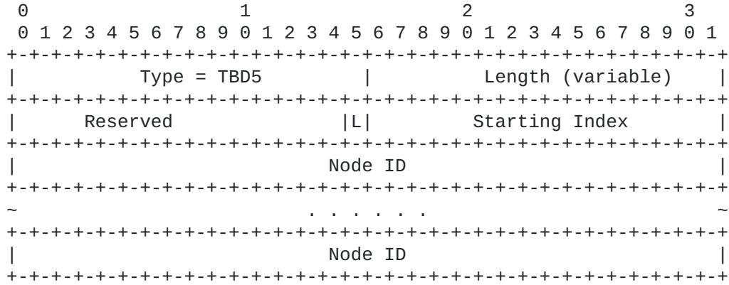
Figure 9: Node IDs TLV
