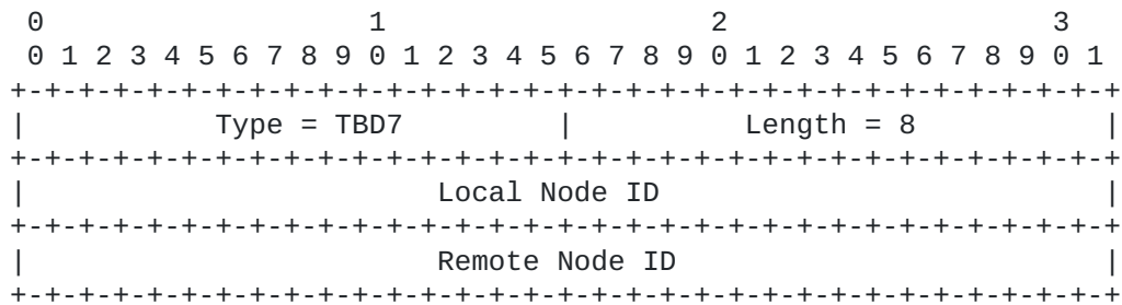
Figure 11: Connection Used for Flooding TLV
