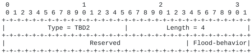
Figure 6: Node Flood TLV
