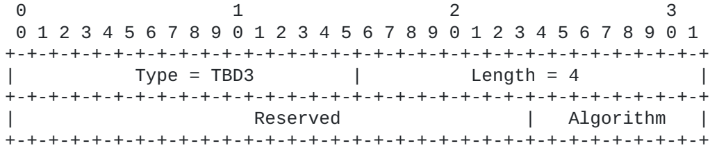
Figure 7: Node Algorithm TLV
