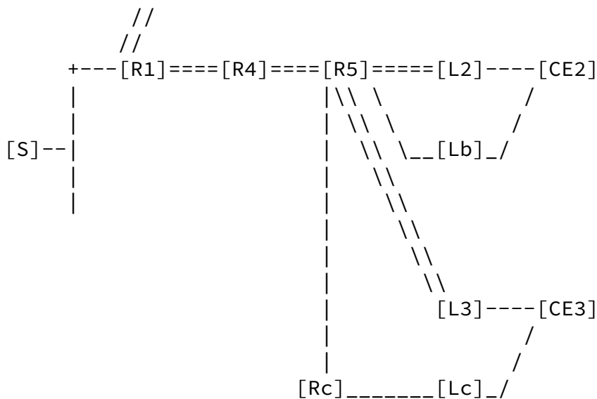
Figure 1: P2MP sub LSP for Locally Protecting Egress
