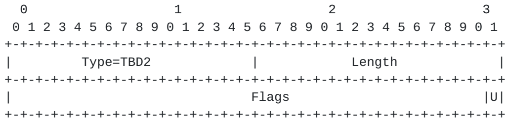
Figure 1: Figure 1 BIER-TE-PCE-CAPABILITY sub-TLV format
