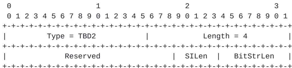
Figure 2: PCE-BIER-TE-Path-Capability sub-TLV
