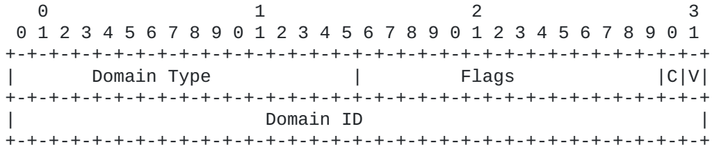
Figure 3: DOMAIN-ID TLV format
