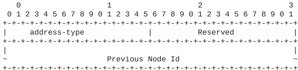
Figure 2: PREVIOUS-NODE TLV format
