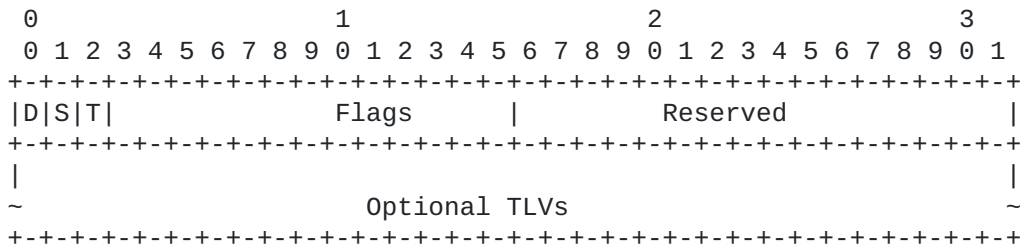
Figure 1: NODE-FLAGS Object Body
