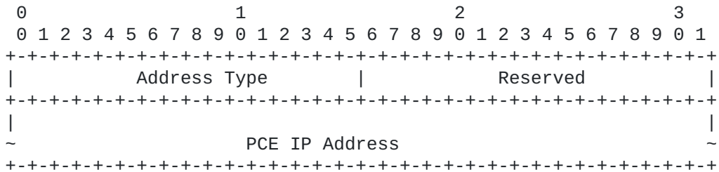
Figure 4: PCE-ID TLV format
