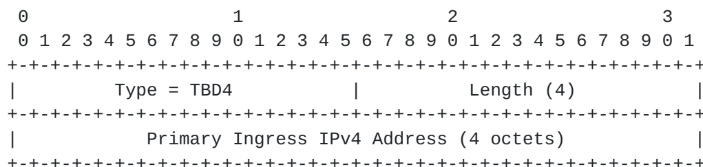
Figure 5: Primary Ingress IPv4 Address sub-TLV
