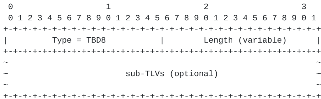
Figure 9: Traffic-Description sub-TLV
