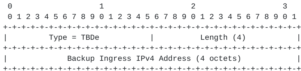
Figure 16: Backup Ingress IPv4 Address TLV
