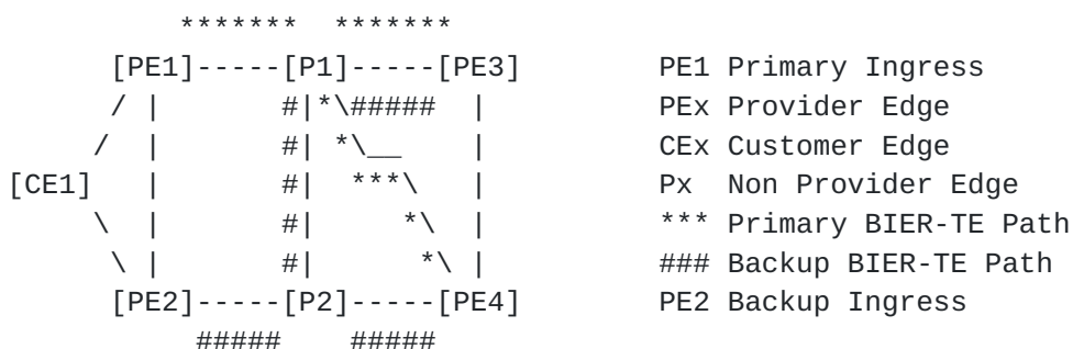
Figure 2: Protecting Ingress PE1 of BIER-TE Path
