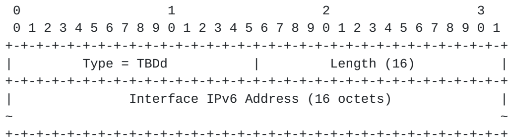
Figure 14: Interface IPv6 Address sub-TLV
