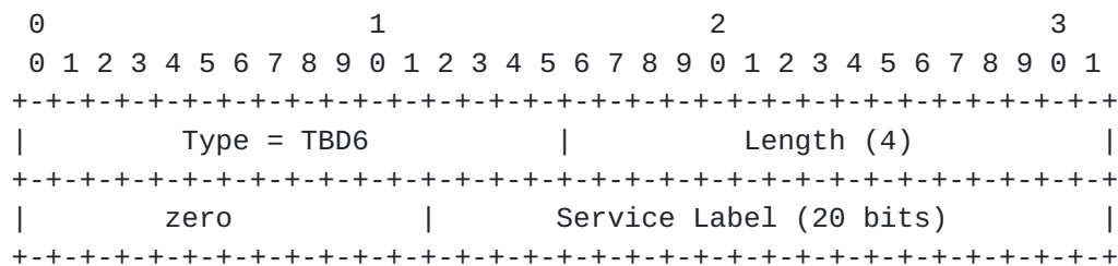
Figure 7: Service Label sub-TLV
