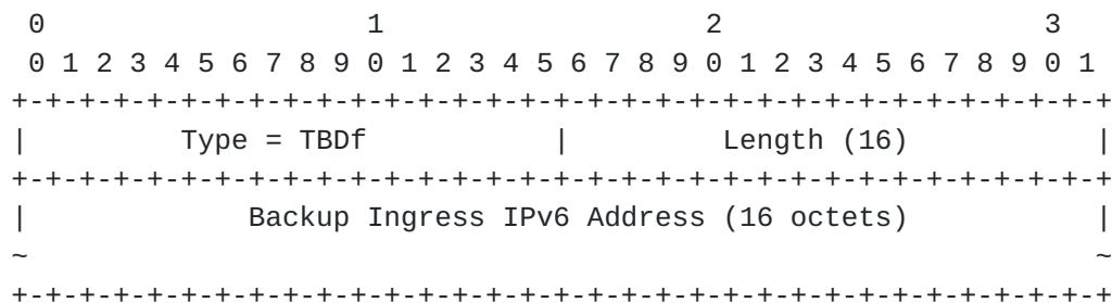
Figure 17: Backup Ingress IPv6 Address TLV
