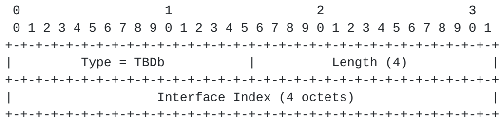
Figure 12: Interface Index sub-TLV
