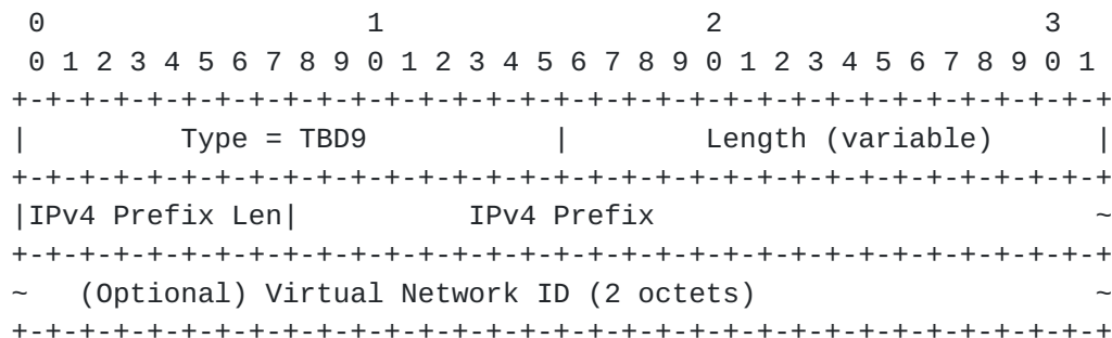
Figure 10: IPv4 FEC sub-TLV
