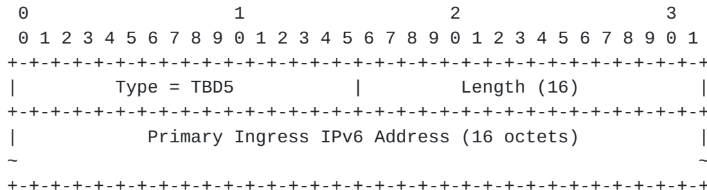
Figure 6: Primary Ingress IPv6 Address sub-TLV
