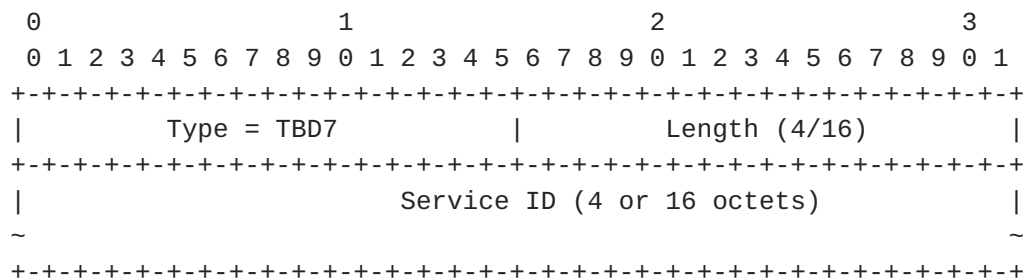
Figure 8: Service ID sub-TLV
