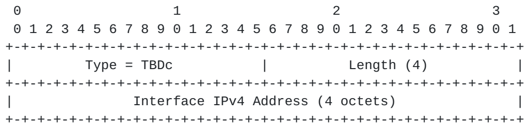
Figure 13: Interface IPv4 Address sub-TLV
