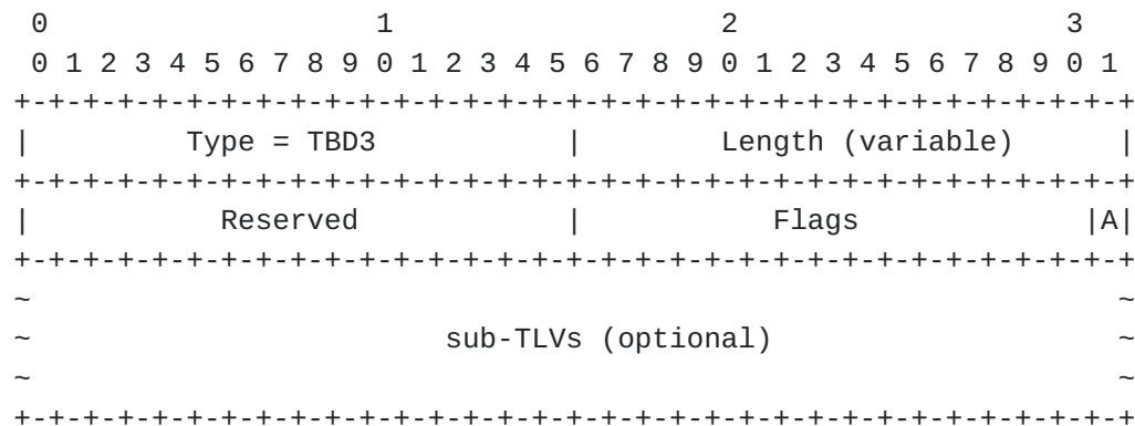
Figure 4: INGRESS_PROTECTION sub-TLV
