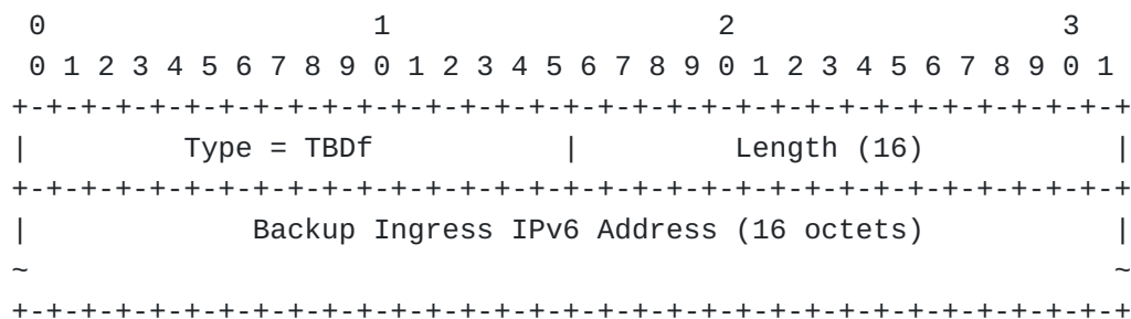
Figure 17: Backup Ingress IPv6 Address TLV
