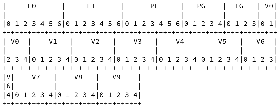
Figure 1: BroadVoice16 bit packing
