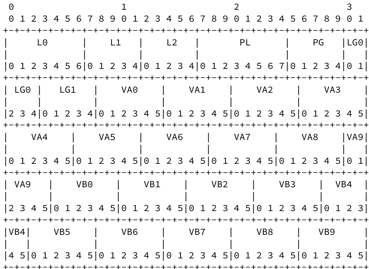
Figure 2: BroadVoice32 bit packing
