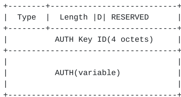
Figure 1: Auth TLV format
