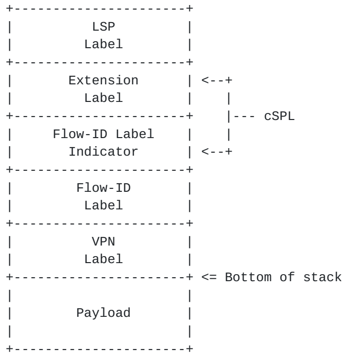
Figure 2: Applying Flow-ID to MPLS LSP
