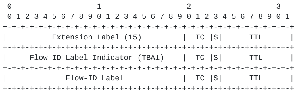
Figure 1: Flow-based PM Encapsulation in MPLS
