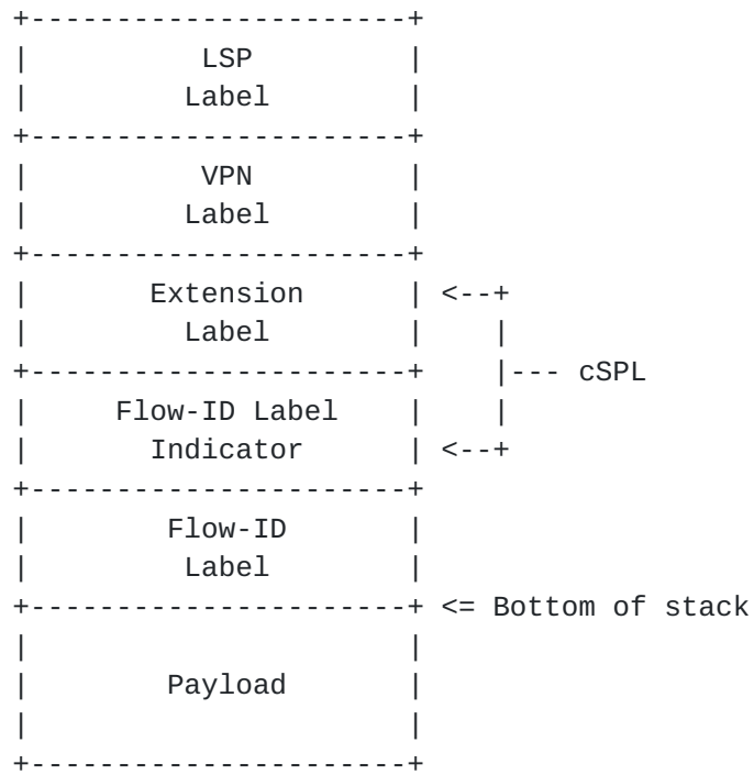
Figure 3: Applying Flow-ID to MPLS VPN
