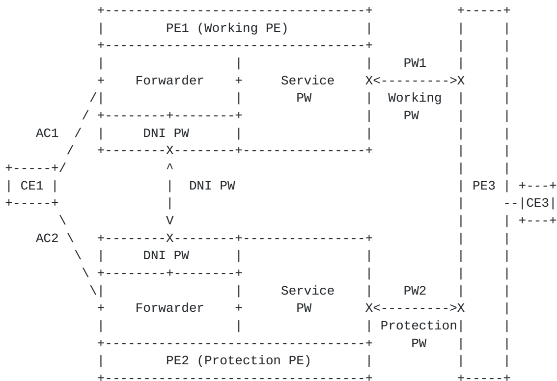
Figure 5. Components of PW dual-homing protection
