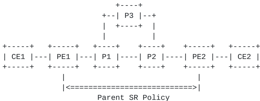
Figure 2 L3VPN over TE Scenario
