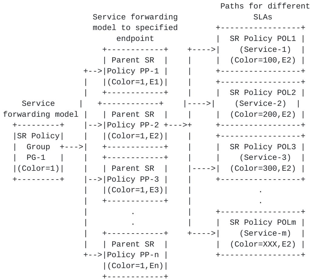
Figure 1 Hierarchical Relationship of SR Policy
