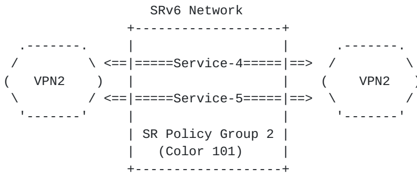
Figure 5 SR Policy Group for VPN2
