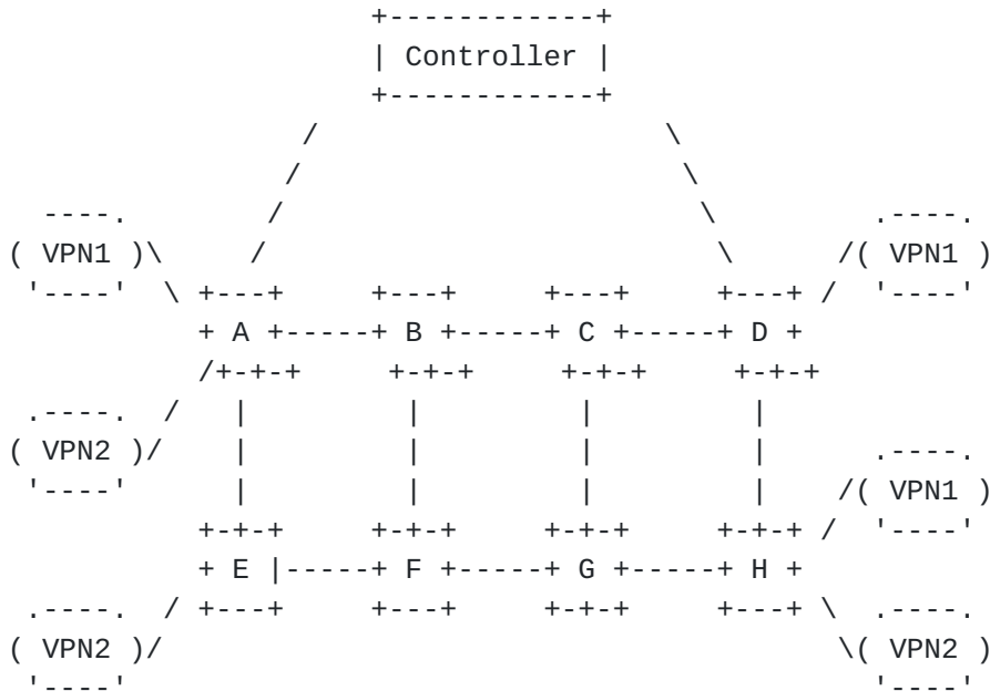
Figure 3 L3VPN over TE application scenario
