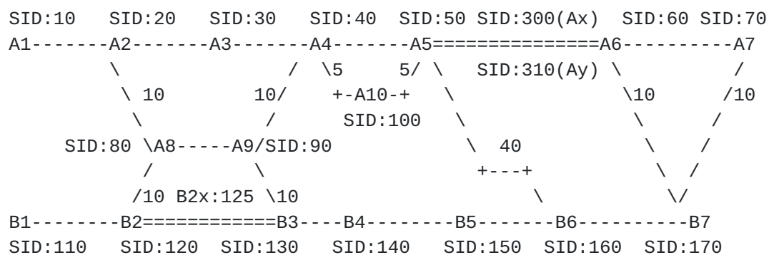
Figure 1: SR-MPLS Network
