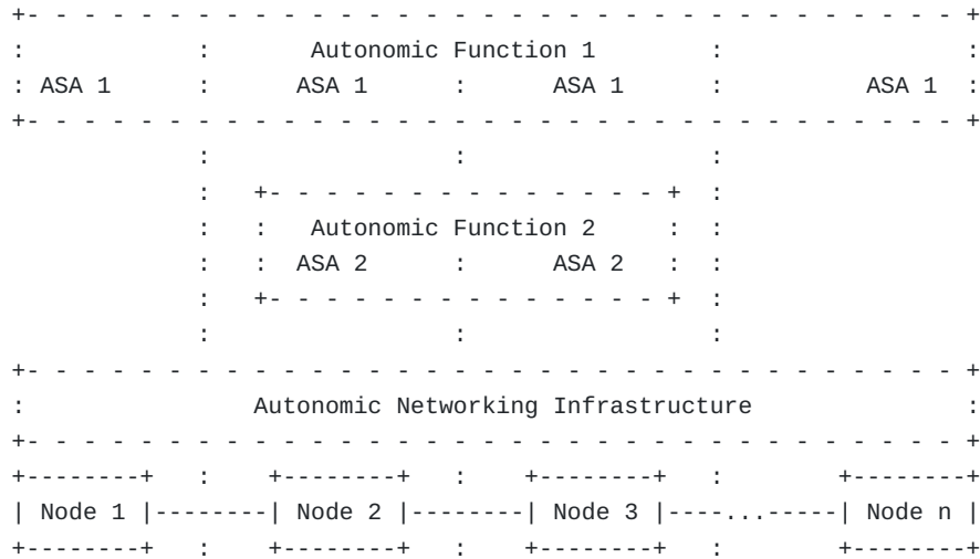
Figure 1: High level view of an Autonomic Network
