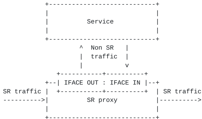
Figure 1: Generic SR proxy
