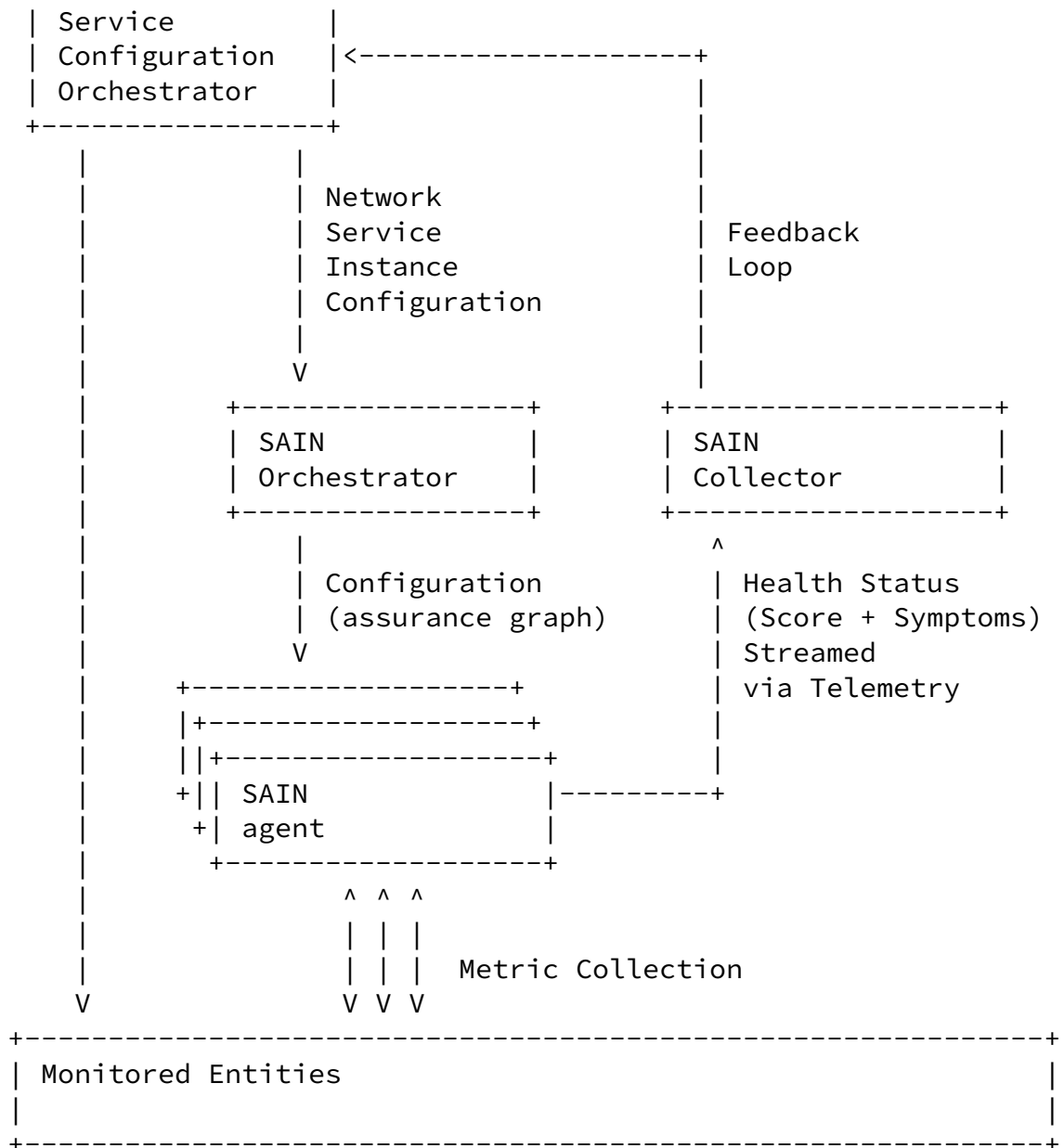
Figure 1: SAIN Architecture
