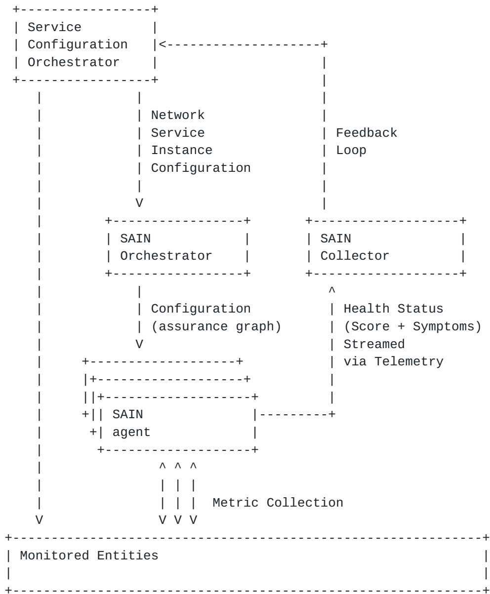
Figure 1: SAIN Architecture
