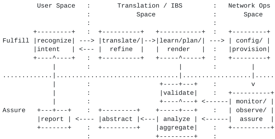
Figure 1: Intent Lifecycle
