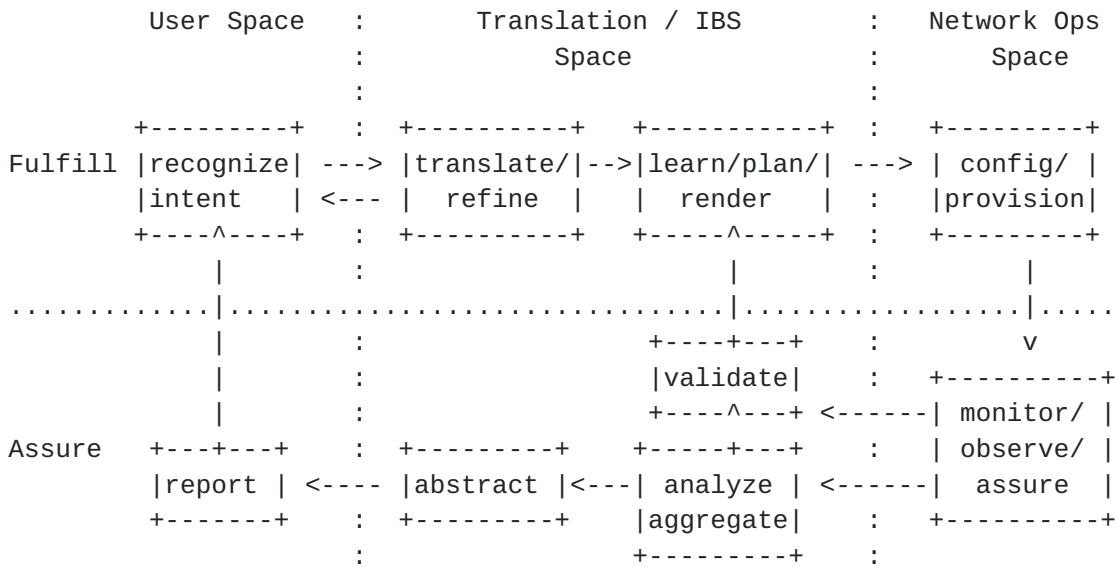
Figure 1: Intent Lifecycle
