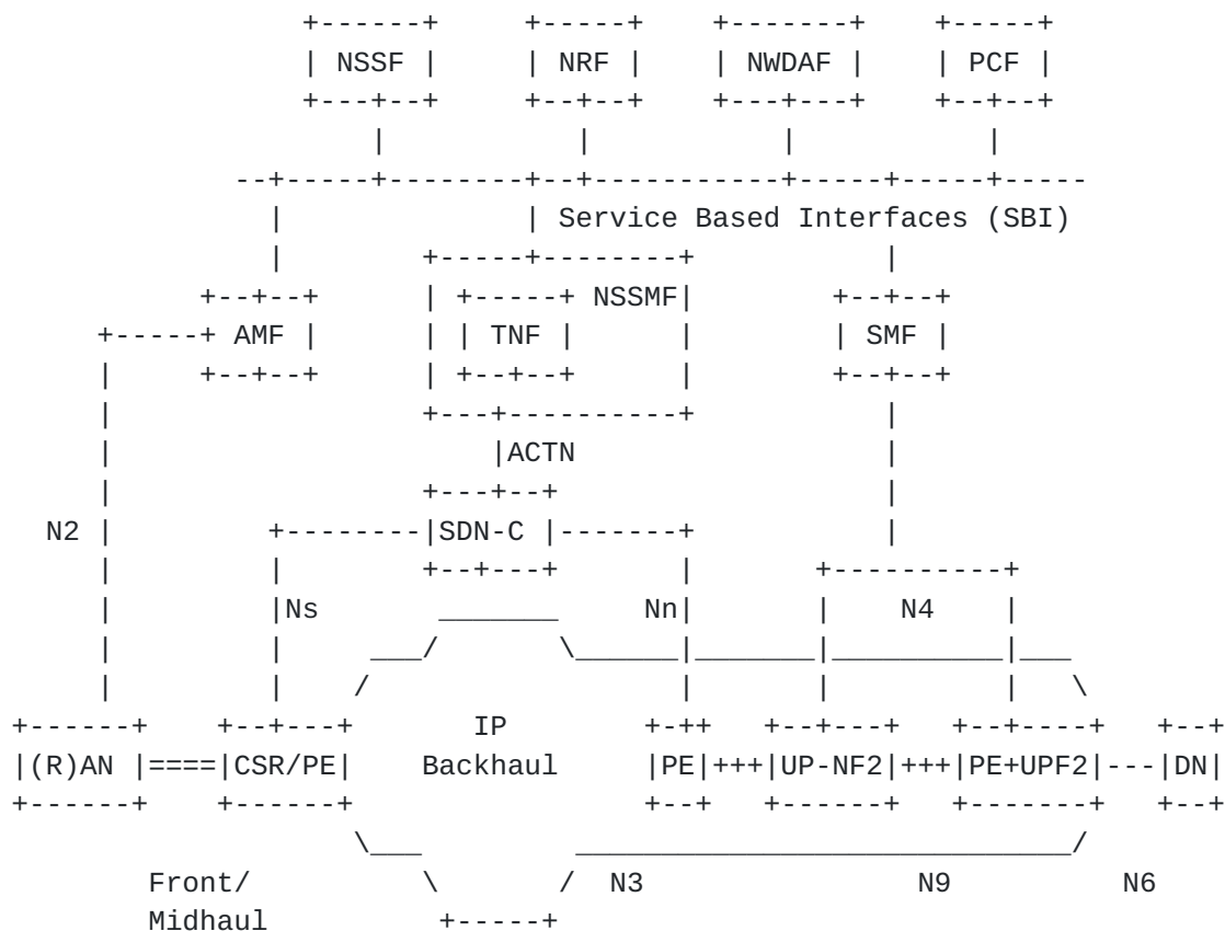
Figure 1: 5G Service Based Architecture with Transport Network
