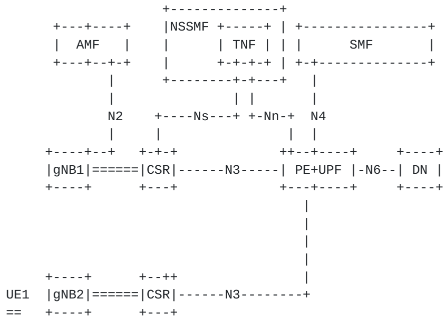
Figure 4: SSC Mode1 with integrated Transport Slice Function
