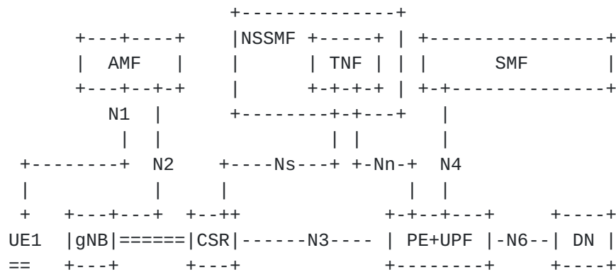
Figure 3: SSC Mode1 with integrated Transport Slice Function
