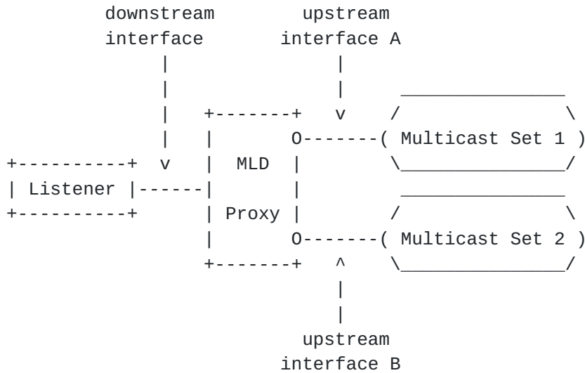
Figure 1: Concept of MLD proxy with multiple upstream interfaces
