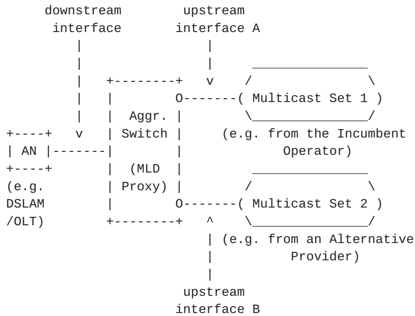
Figure 2: Example of usage of an MLD proxy with multiple upstream interfaces in a fixed network scenario
