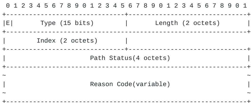
Figure 2: Encoding of IANA-Registered Path Status TLV
