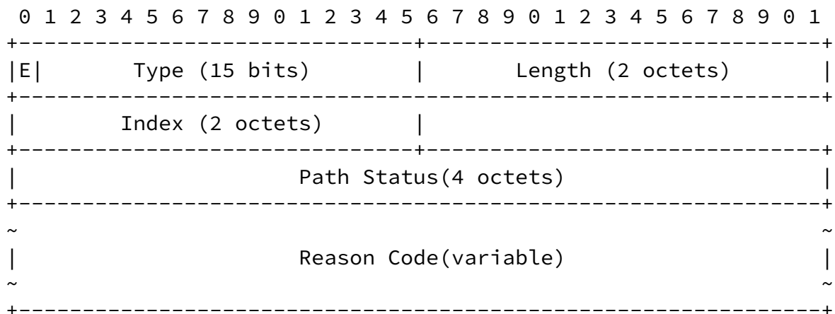
Figure 2: Encoding of IANA-Registered Path Status TLV
