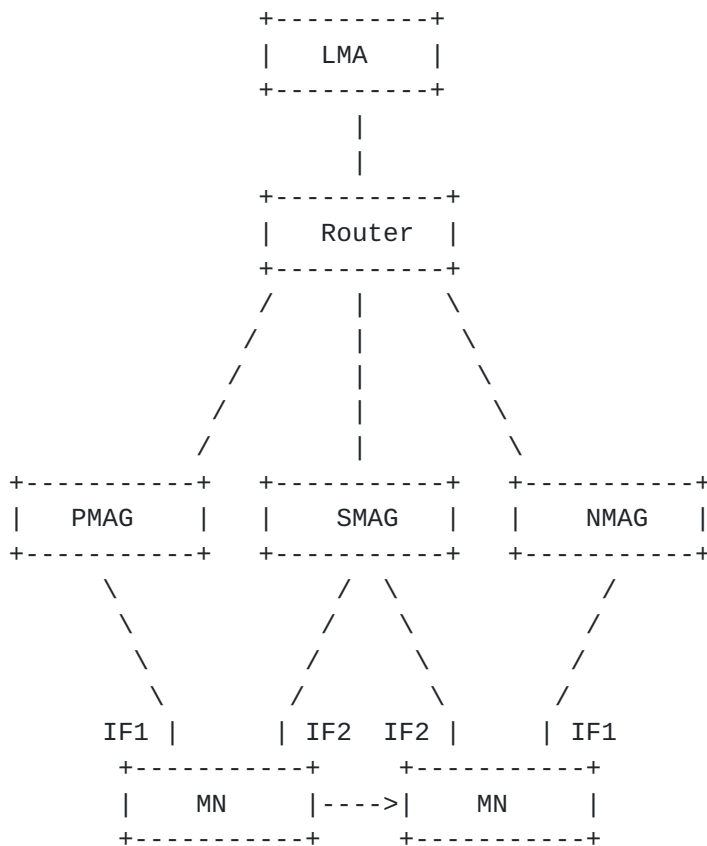
Figure 1 reference network for Multiple-Access Mobile Node handover
