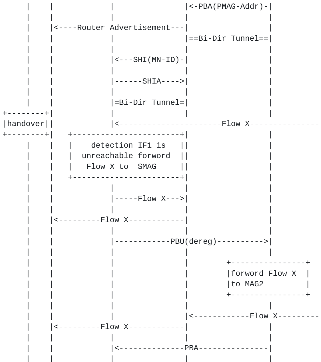
Figure 2 the signaling process of streamless handover scheme for Multiple-Access Mobile Node
