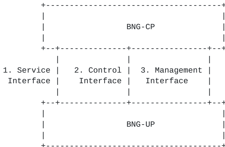
Figure 2. Internal Interfaces Between the BNG CP and UP
