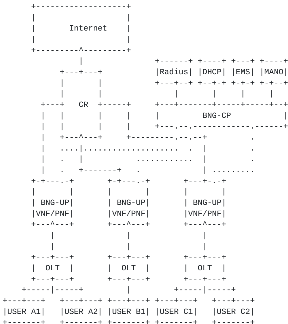
Figure 3: Cloud BNG Deployed in Several Districts
