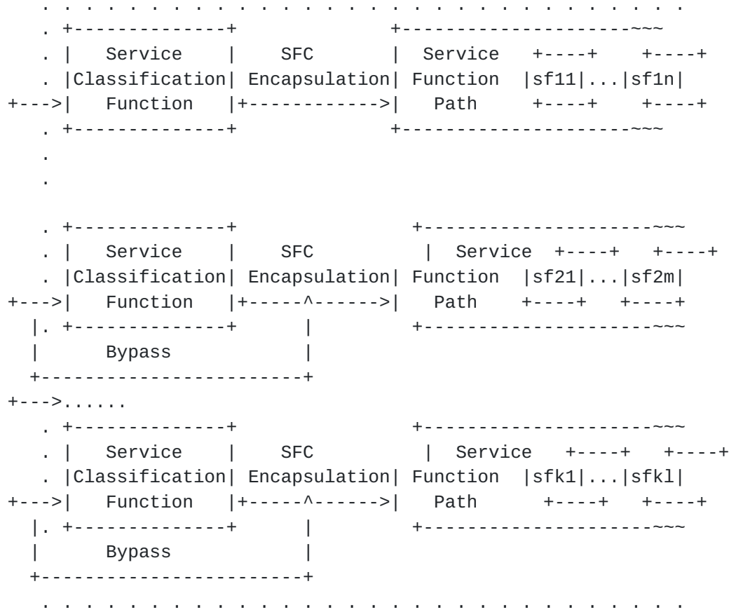
Figure 3: General architecture for fused service function chain
