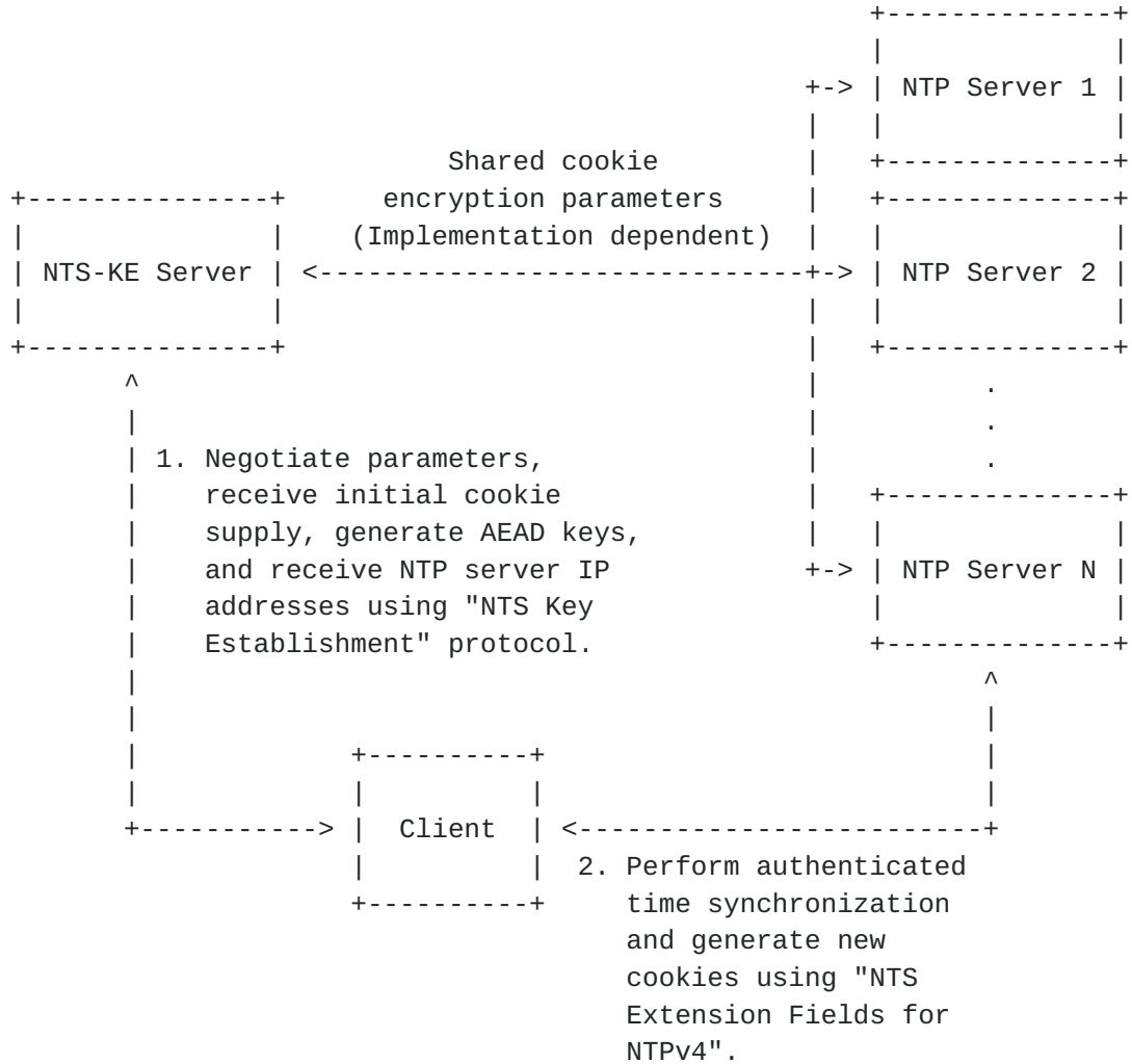
Figure 1: Overview of High-Level Interactions in NTS
