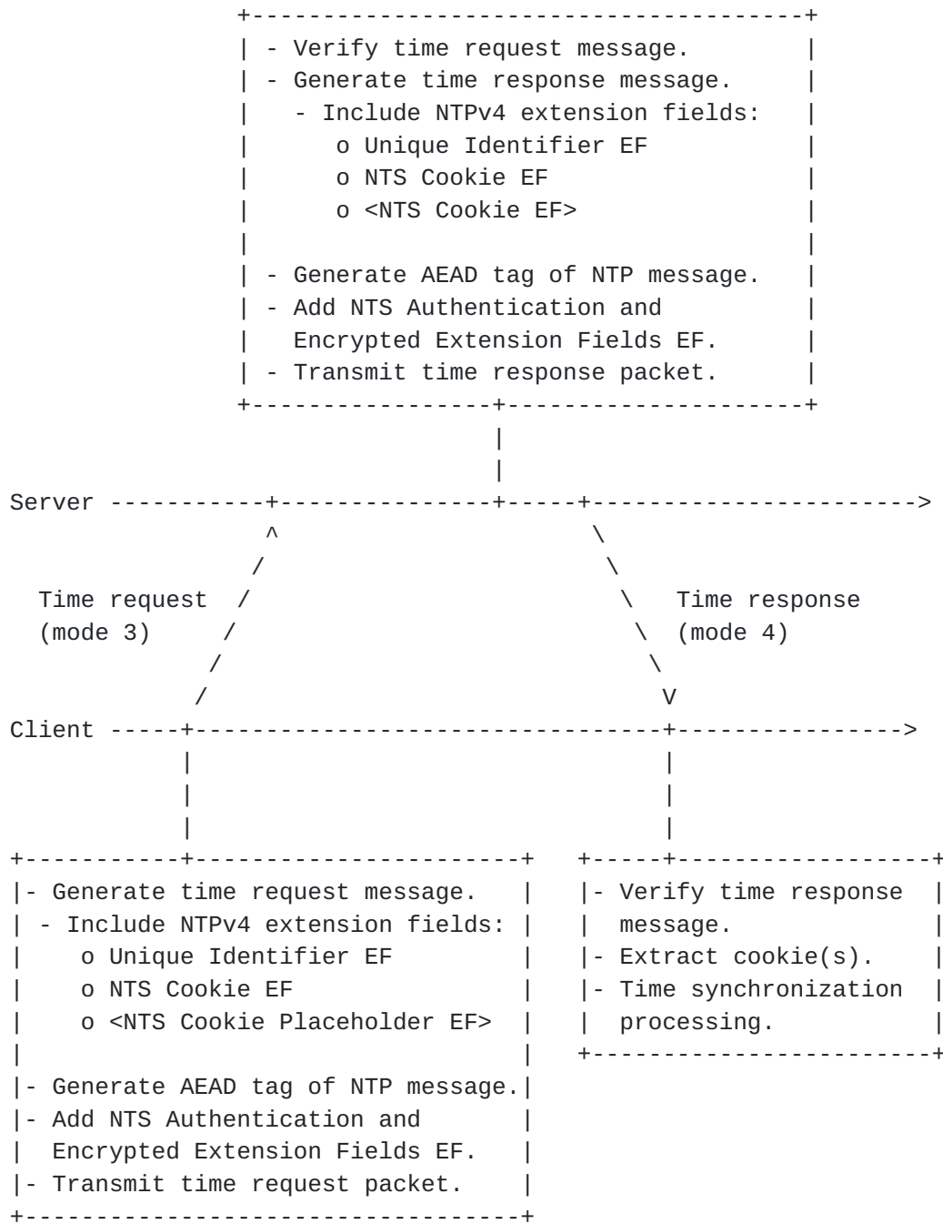
Figure 5: NTS Time Synchronization Messages
