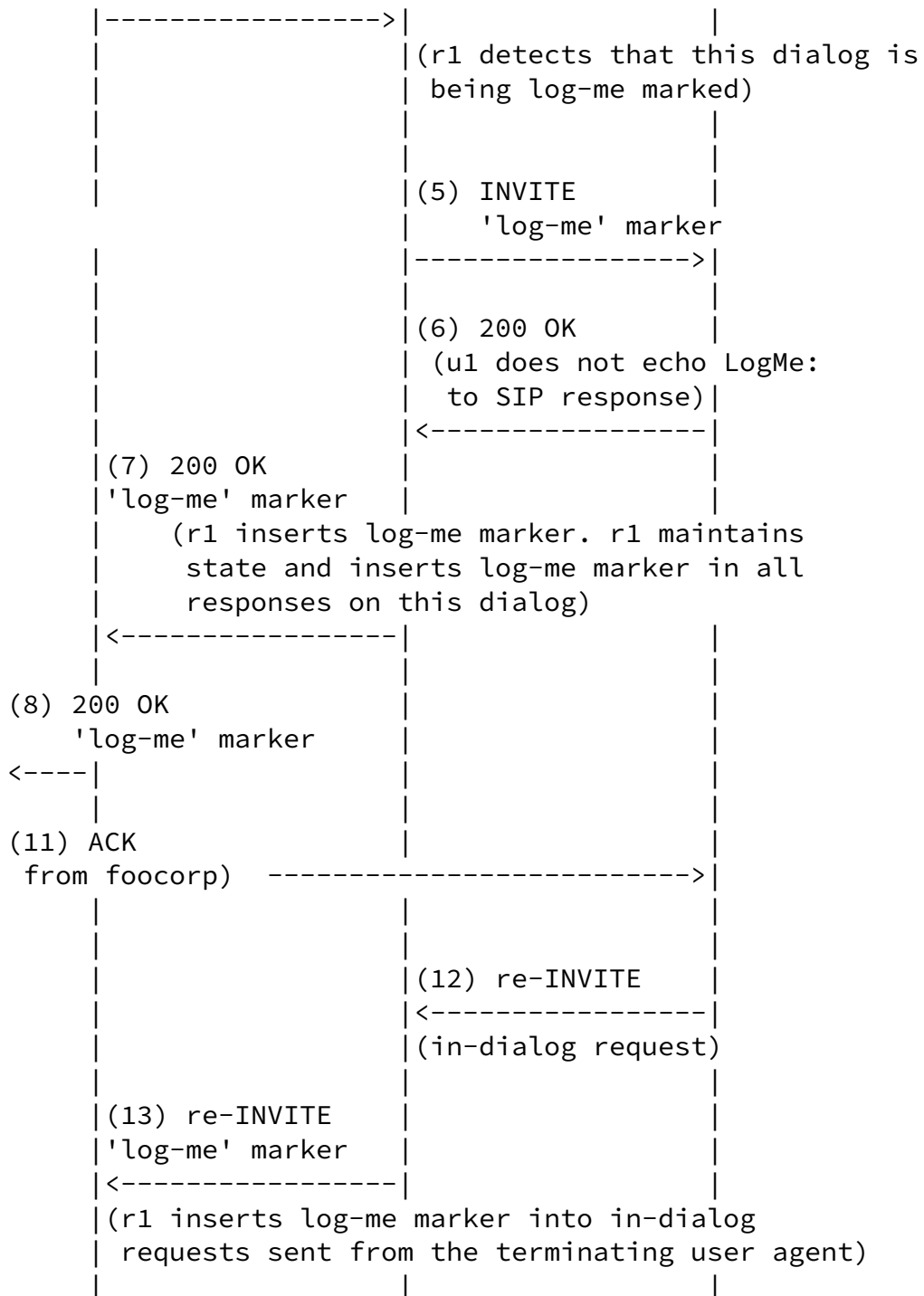
Figure 3: Maintaining state for log-me marking
