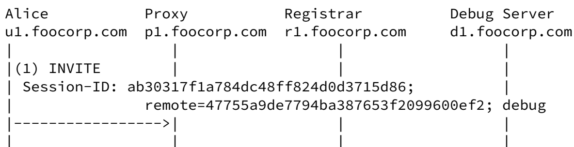
Figure 4: Log-me marking using the "debug" Session-ID: header field parameter
