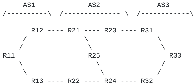
Figure 1: end-to-end SRLG protection
