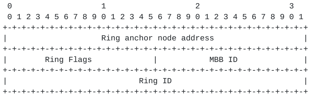
SESSION Object
