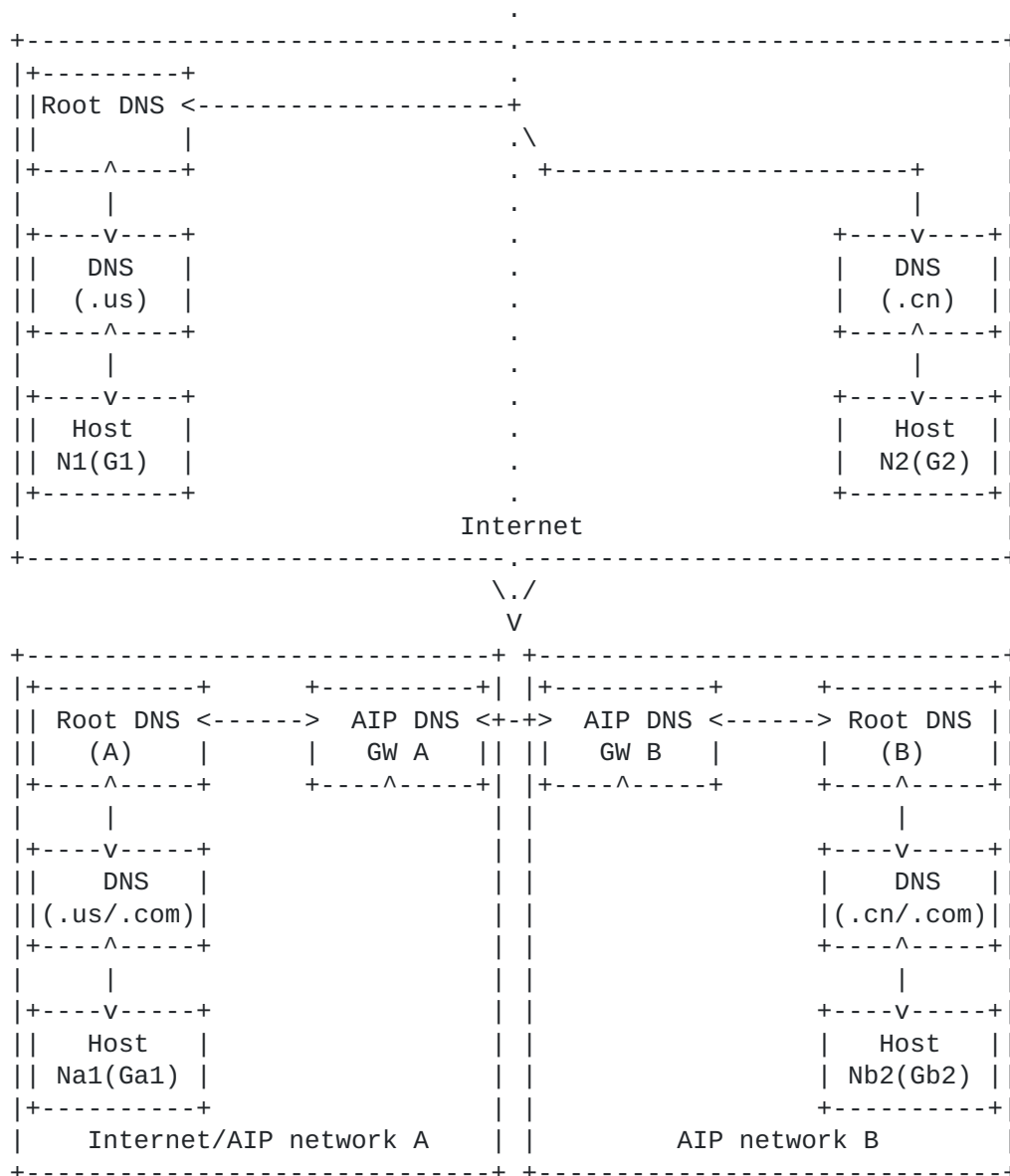
Figure 2: AIP DNS architecture and transformation
