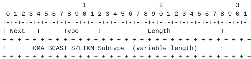
Figure 1: OMA BCAST MIKEY General Extension
