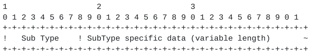
Figure 2: STKM/LTKM Subtype Payload
