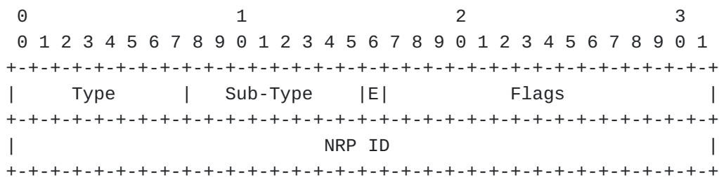
Figure 1. The format of Encapsulate-NRP-ID action
