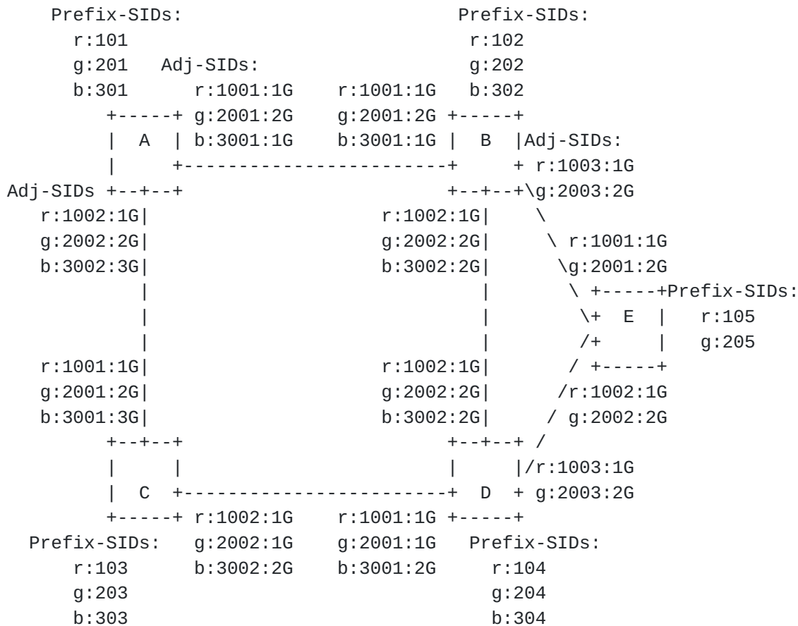
Figure 1. SID and resource allocation for multiple VTNs
