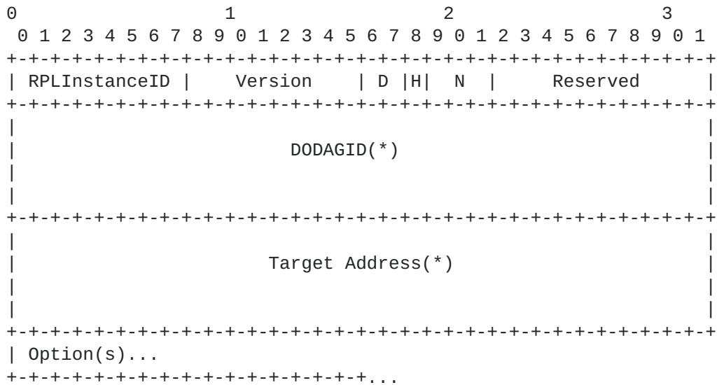
Figure 2: Format of the Discovery Reply Object (DRO)
