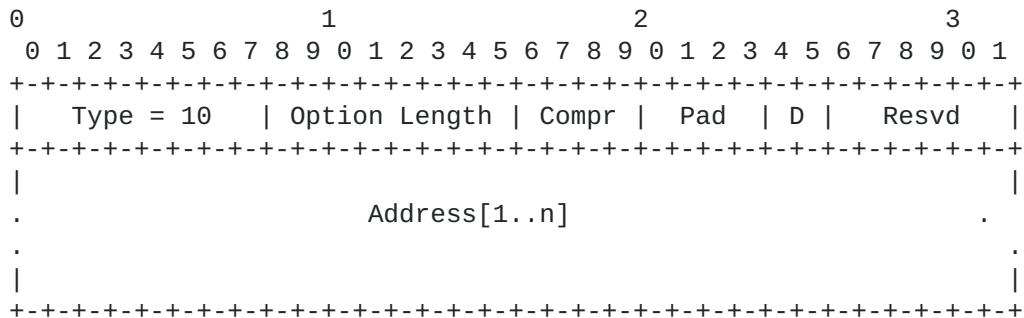
Figure 3: Format of the Source Route Option
