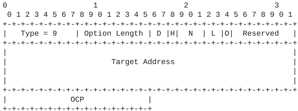
Figure 1: Format of the Route Discovery Option
