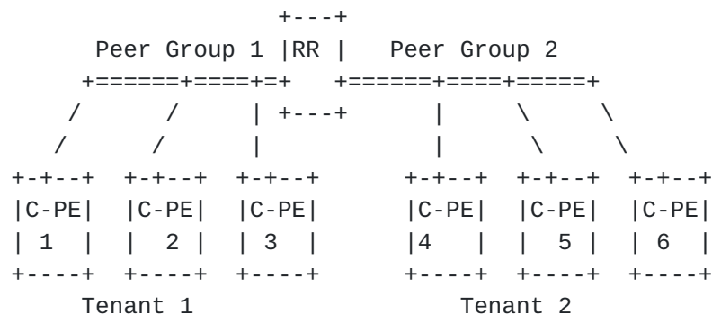
Figure 1: Peer Groups managed by Local Controller
