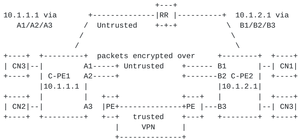
Figure 9: SDWAN Scenario #2 WAN Ports Registration
