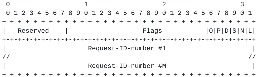
Figure 1: SVEC Body Object Format
