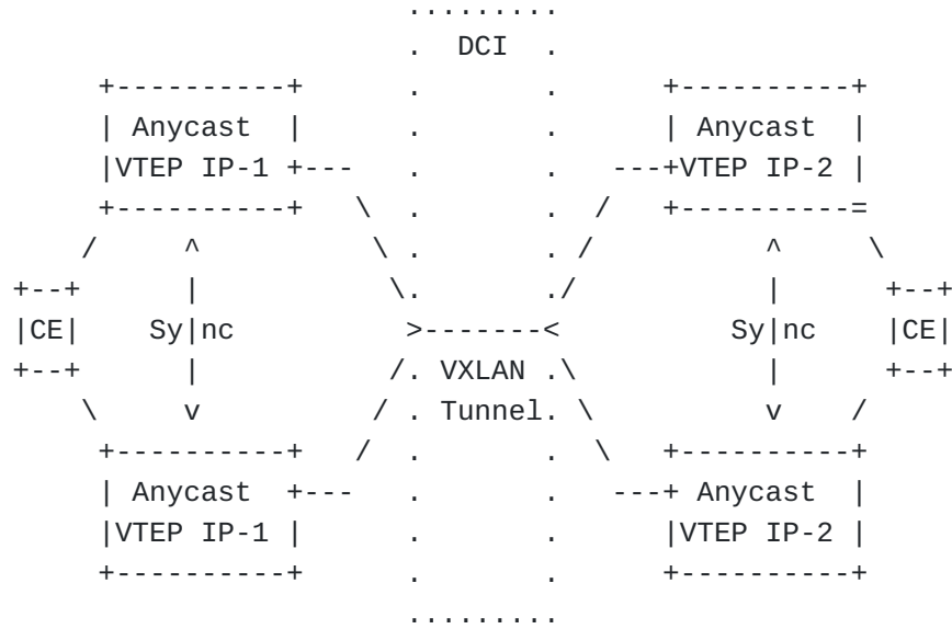
Figure 2: Situation Using Anycast
