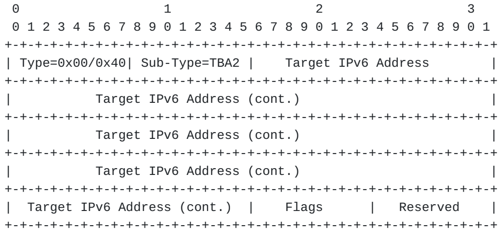
Figure 5: IPv6-address-specific Bypass VXLAN Extended Community
