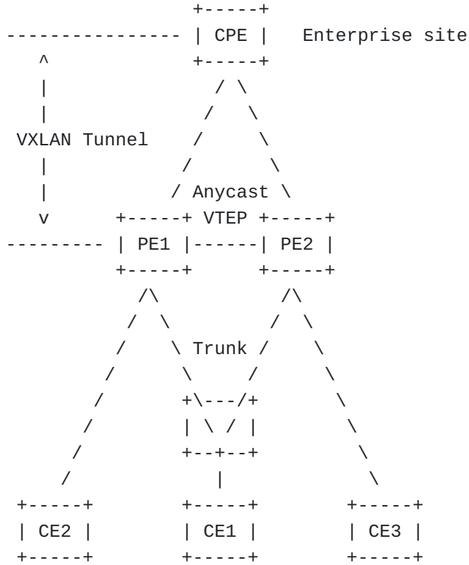
Figure 3: Basic networking of the VXLAN active-active scenario
