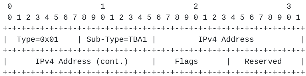
Figure 4: IPv4-address-specific Bypass VXLAN Extended Community
