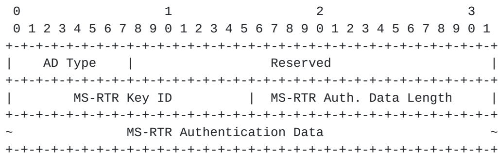
Changes to LISP Map-Notify Message
