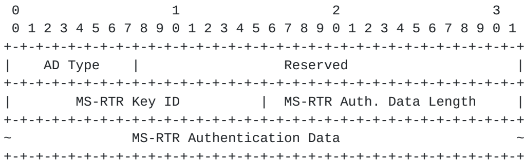
Changes to LISP Map-Notify Message
