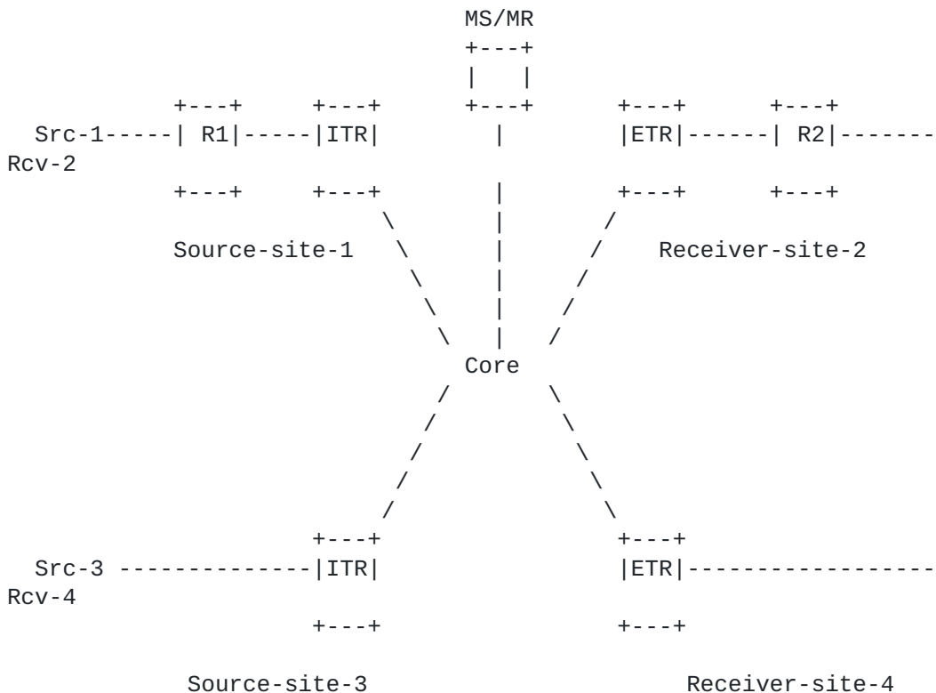
Figure 1: LISP Multicast Generic Reference Model
