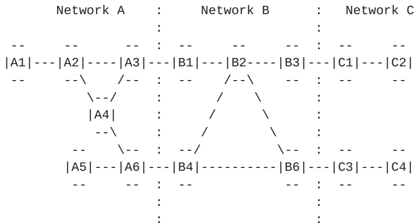
Figure 16 : A Network Comprising Three Peer Networks
